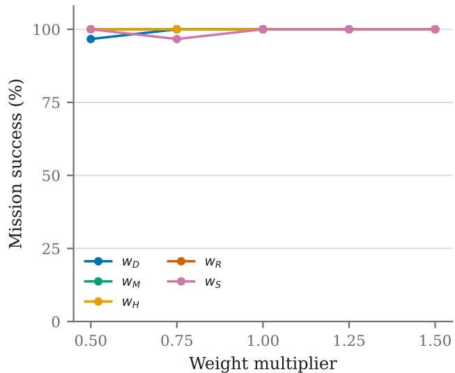
(a) Success
