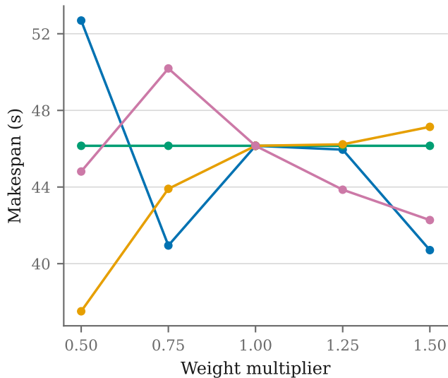
(b) Makespan
