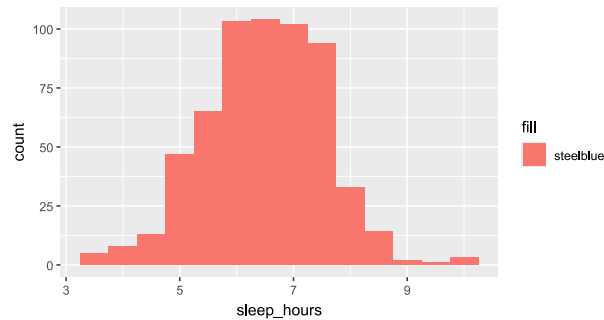
Figure 4.11: The mistake: a fixed colour inside aes() is treated as data.
