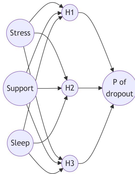
Figure 15.1: A neural network with one hidden layer. Every arrow carries a weight; each hidden neuron and the output neuron add up their weighted inputs and apply an activation function.
