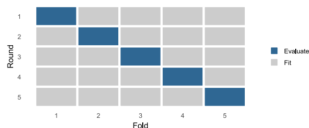
Figure 11.4: Five-fold cross-validation: in each round, the model is fitted on four folds (grey) and evaluated on the fifth (dark).
