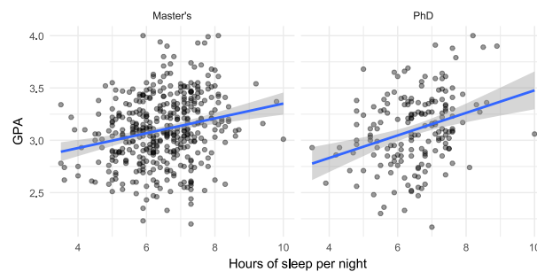
Figure 4.18: Sleep and GPA in the first semester, one panel per programme.
