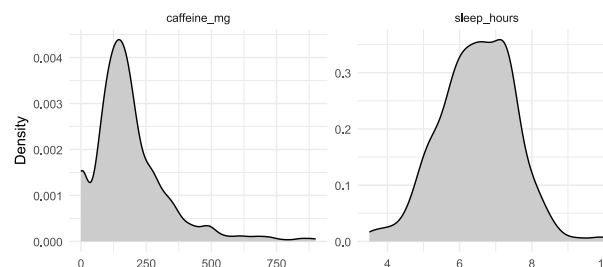
Figure 6.4: Sleep is roughly symmetrical; caffeine is skewed to the right.
