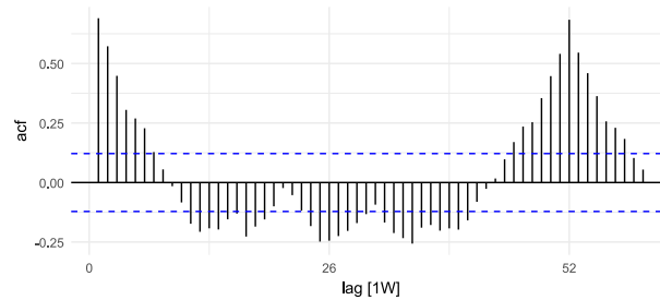
Figure 16.5: Autocorrelation of weekly visits for lags of 1 to 60 weeks. The dashed lines mark the range expected for a series with no autocorrelation.
