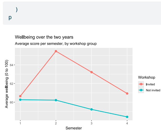
Figure 4.12: The line chart with clear labels.
