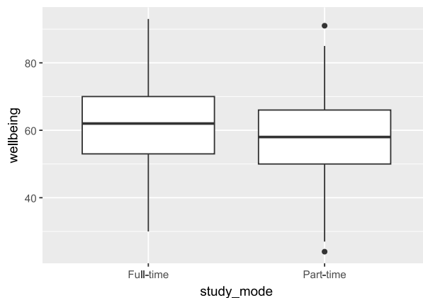
Figure 4.7: Wellbeing in the first semester, by study mode.
