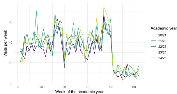
Figure 16.3: Seasonal plot: weekly visits by week of the academic year, one line per year.
