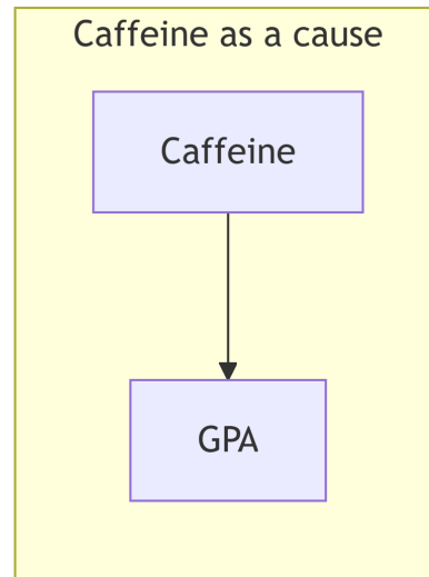
Figure 8.5: Two explanations for the link between caffeine and GPA. Left: caffeine affects GPA. Right: sleep affects both caffeine and GPA, which creates a link between them even if caffeine has no effect.
