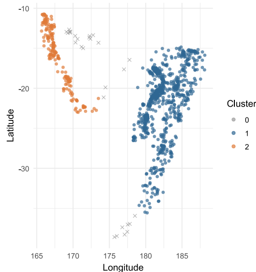
Figure 14.6: Earthquakes near Fiji, clustered by DBSCAN. Grey crosses are noise.
