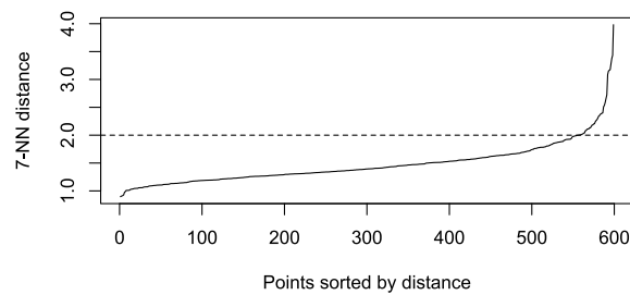
Figure 14.5: Distance from each student to their seventh-nearest neighbour, sorted. The dashed line marks \text{eps} = 2 .
