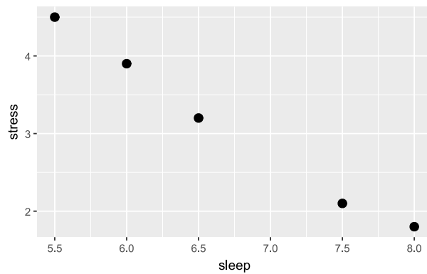
Figure 4.4: Adding a layer of points: students who sleep less report more stress.
