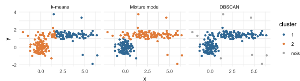
Figure 14.1: The same simulated data clustered by k-means, a Gaussian mixture model, and DBSCAN. The data contains a round group, a long thin group, and scattered points that belong to neither; each method's definition of a group decides what it finds.
