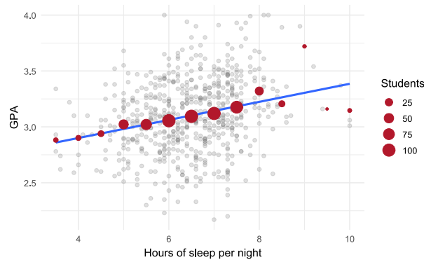
Figure 8.4: GPA and sleep. Grey points are students; red points are the average GPA in each half-hour band of sleep, sized by the number of students; the line is the linear regression. The line is a smooth summary of the red averages.
