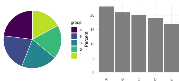
Figure 4.2: The same five percentages as a pie chart (angles and areas) and as a bar chart (lengths on a common scale). The order of the groups is much easier to see in the bars.
