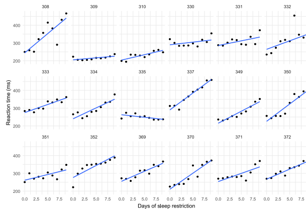
Figure 10.1: Reaction times over 10 days of sleep restriction, one panel per person, with each person's own trend line.
