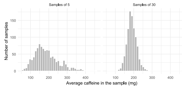
Figure 7.1: The sampling distribution of average caffeine intake, for samples of 5 and of 30 students drawn from the student wellbeing data.
