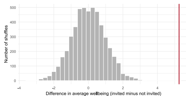
Figure 7.2: The null distribution from 5,000 shuffles of the workshop labels, and the observed difference (red line). No shuffle came close to the observed difference.
