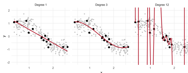
Figure 11.1: Three models fitted to the same 15 training points (black). The straight line is too simple, the degree-3 curve follows the pattern, and the degree-12 curve passes close to every training point but wanders far from the new points (grey).
