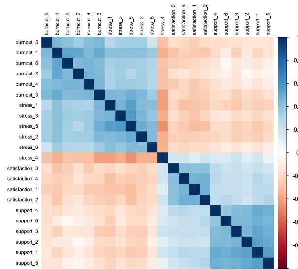
Figure 9.1: Correlations among the 22 questionnaire items, sorted so that similar items are next to each other.
