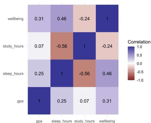
Figure 4.20: Correlations between four first-semester measurements.
