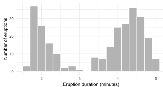
Figure 6.7: Old Faithful eruption durations: a bimodal distribution.
