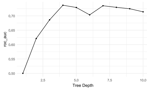
Figure 11.5: Cross-validated ROC AUC of decision trees of different depths.
