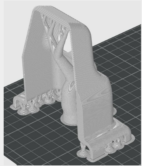
Grip Shell (+Brim recommended)
