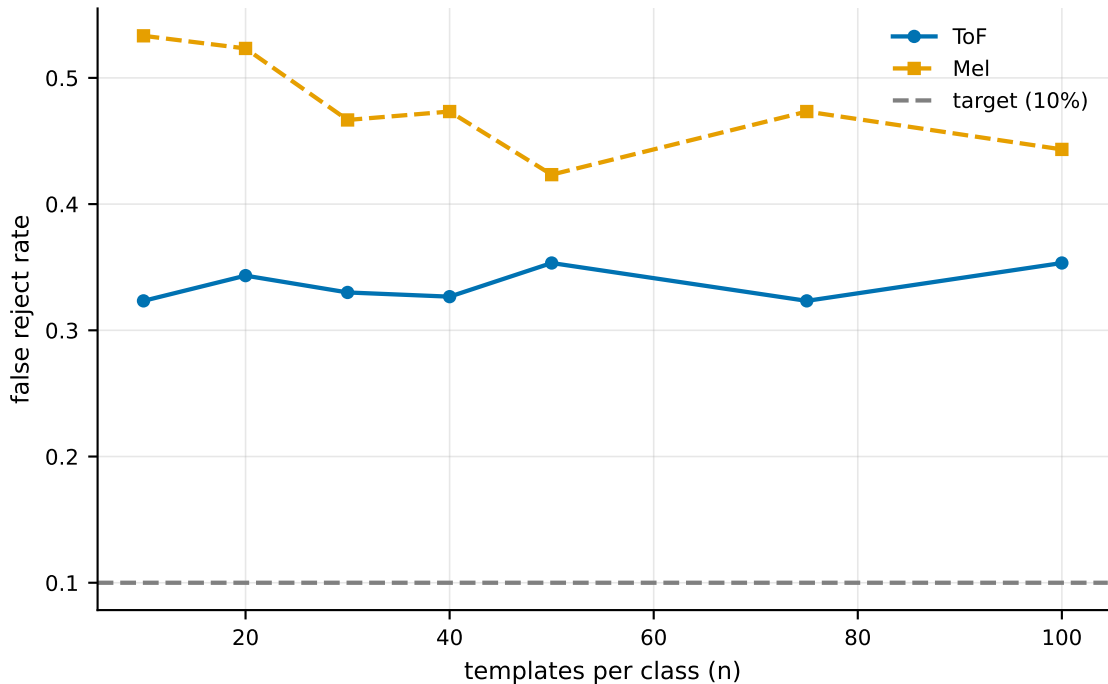
False reject rate vs template count (synthetic, real-scale)
