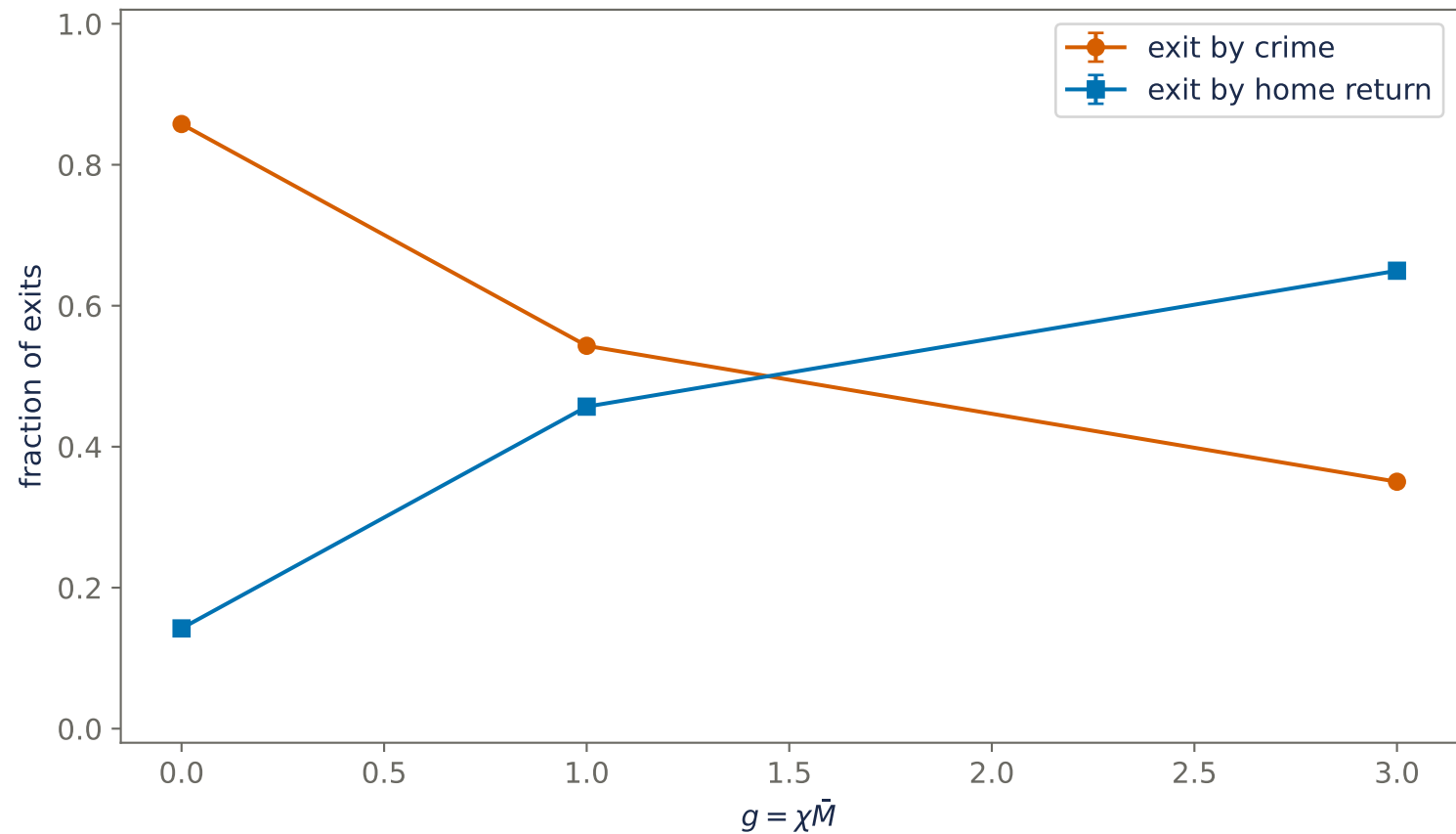
Exit-channel split vs g (mean \pm SEM over seeds)
