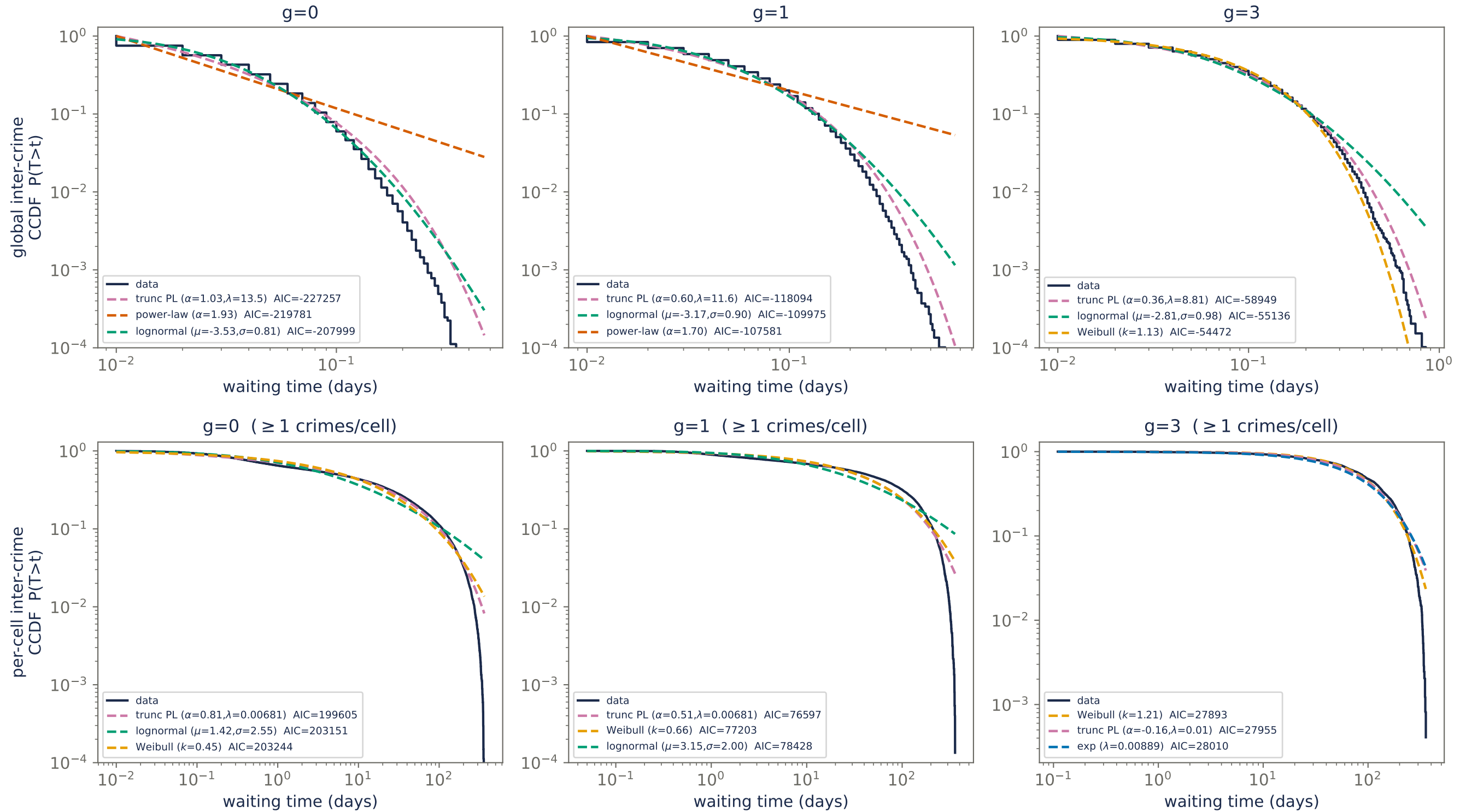
Inter-crime CCDFs with best-fit laws (dashed = top-3 by AIC; full ranking in waiting_times_fits.csv)
