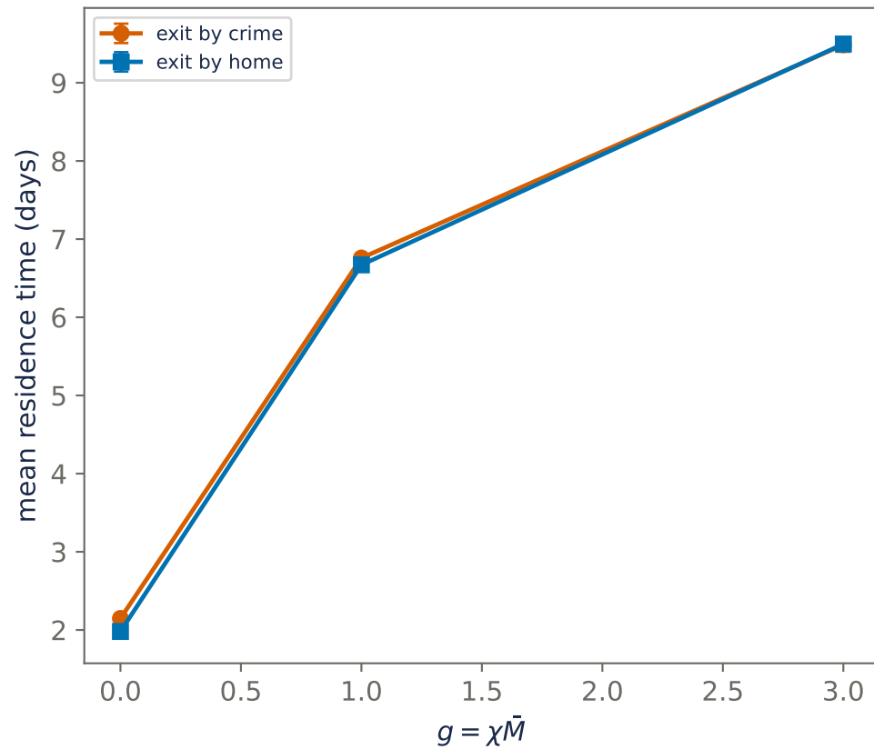
Waiting & residence times vs g (mean \pm SEM over seeds; CV > 1 = bursty, CV \approx 1 = Poisson)
