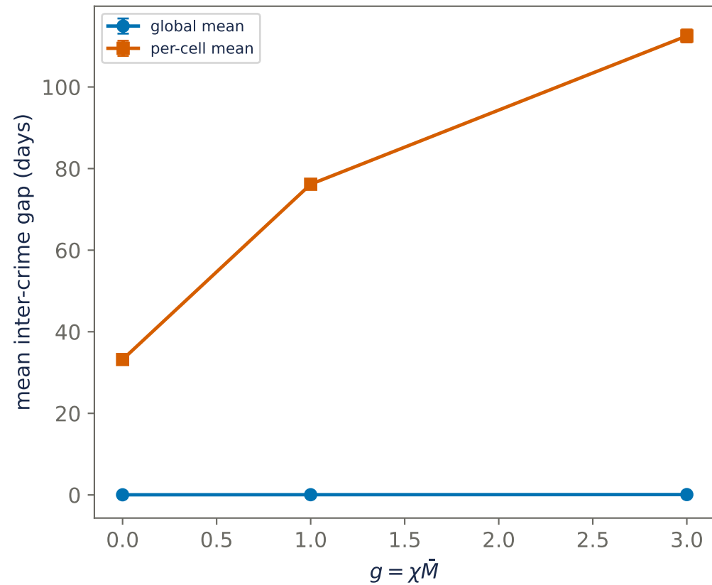
Waiting & residence times vs g (mean \pm SEM over seeds; CV > 1 = bursty, CV \approx 1 = Poisson)
