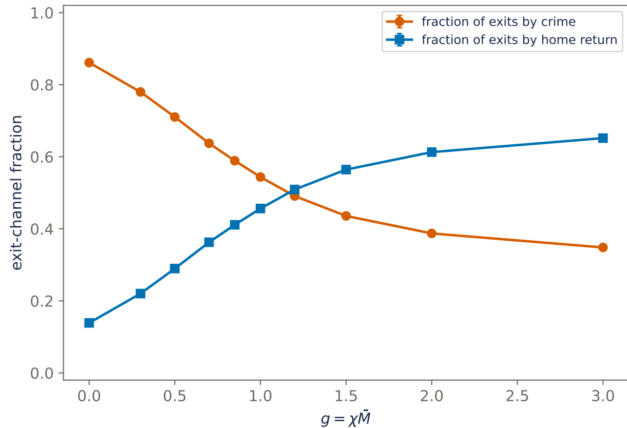
Exit channels vs g: as deterrence rises, crime gives way to home exits
