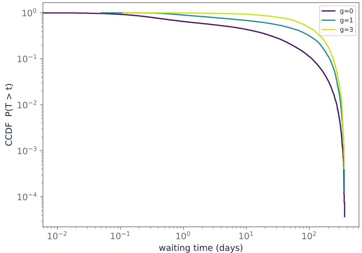
Per-cell inter-crime gap (repeat victimization; \geq 1 crime/cell)
