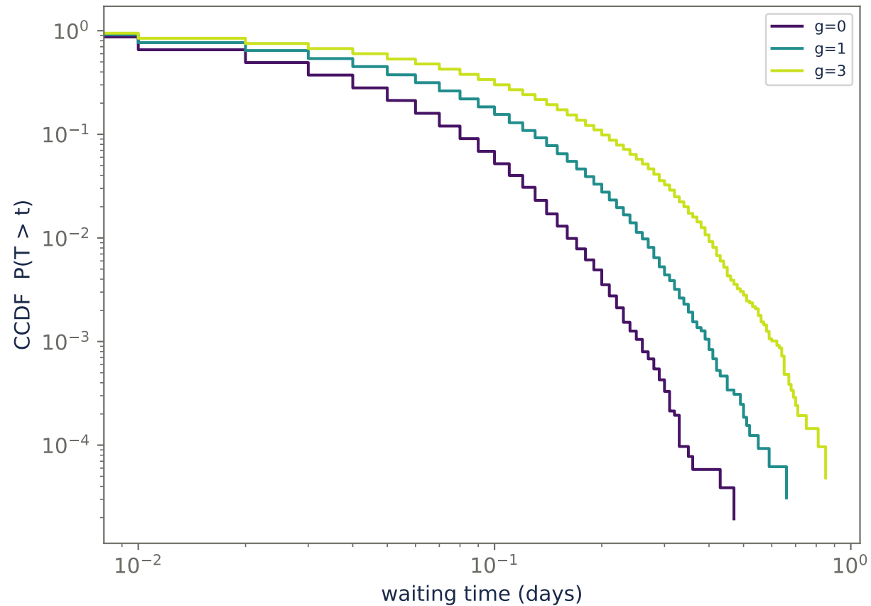
Global inter-crime gap (gaps lengthen as g rises: crime slows)
