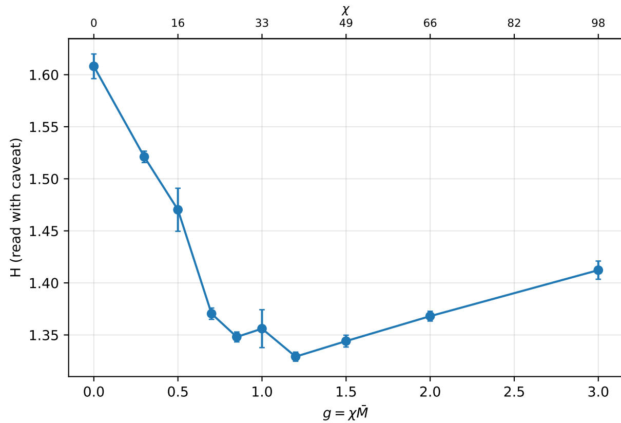
Hotspot order parameters vs g (return-home, \delta = 1/15 ; mean \pm SEM over seeds)
