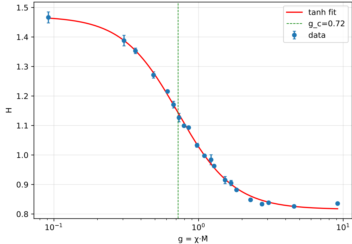
Focused transition: tanh crossover fit (mean \pm SEM over seeds)
