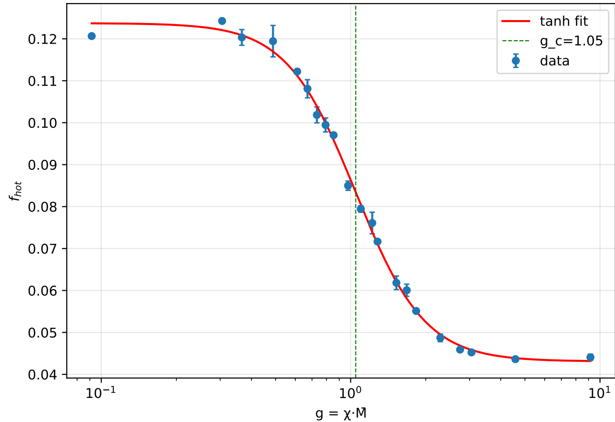
Focused transition: tanh crossover fit (mean \pm SEM over seeds)
