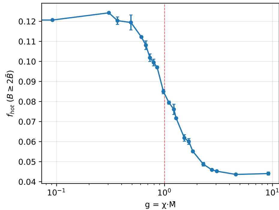
Transition order parameters vs g (B+C combined, mean \pm SEM over seeds)
