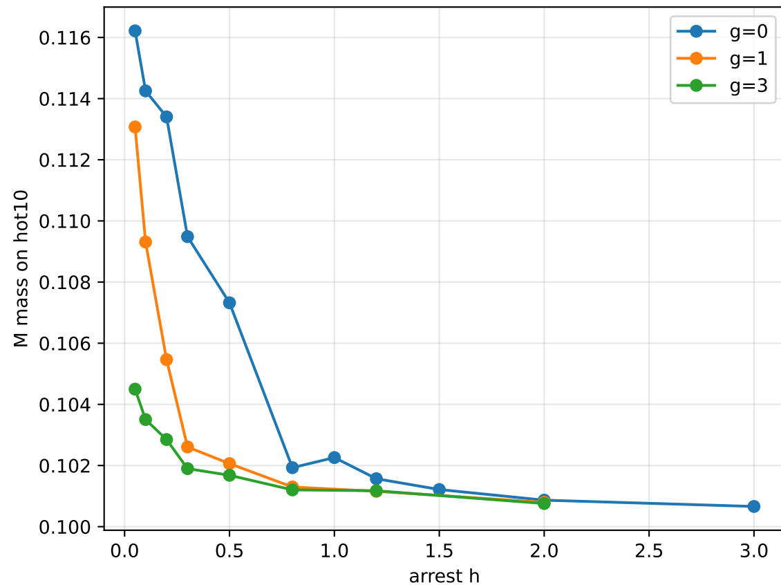
Arrest feedback: as crime collapses, police field M de-concentrates \rightarrow arrest tends to uniform
