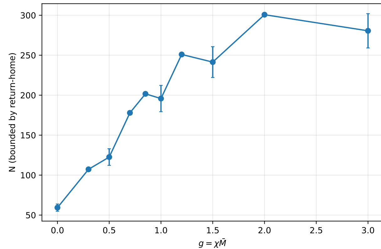
Transition summary vs g : bounded N , falling crime, hotspots dissolve
