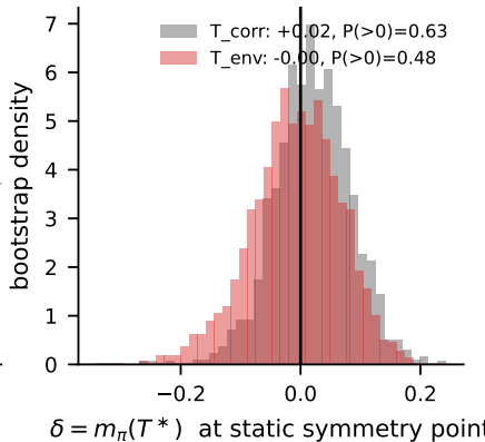
paired walk-stratified bootstrap
