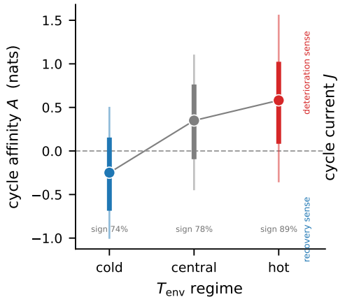
(a) detailed-balance breaking
