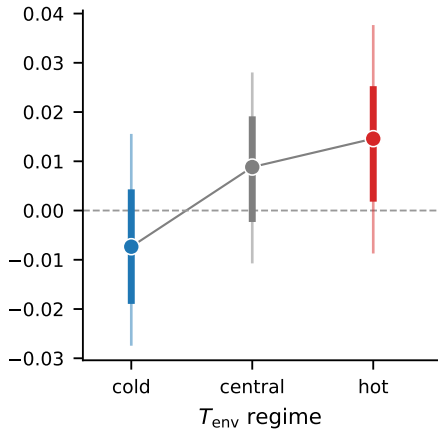
(b) net cycle current
