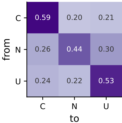
aggregate P_{ij}
