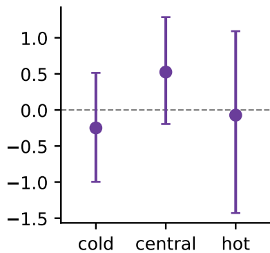
detailed-balance breaking
