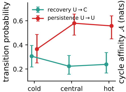
kinetic mechanism
