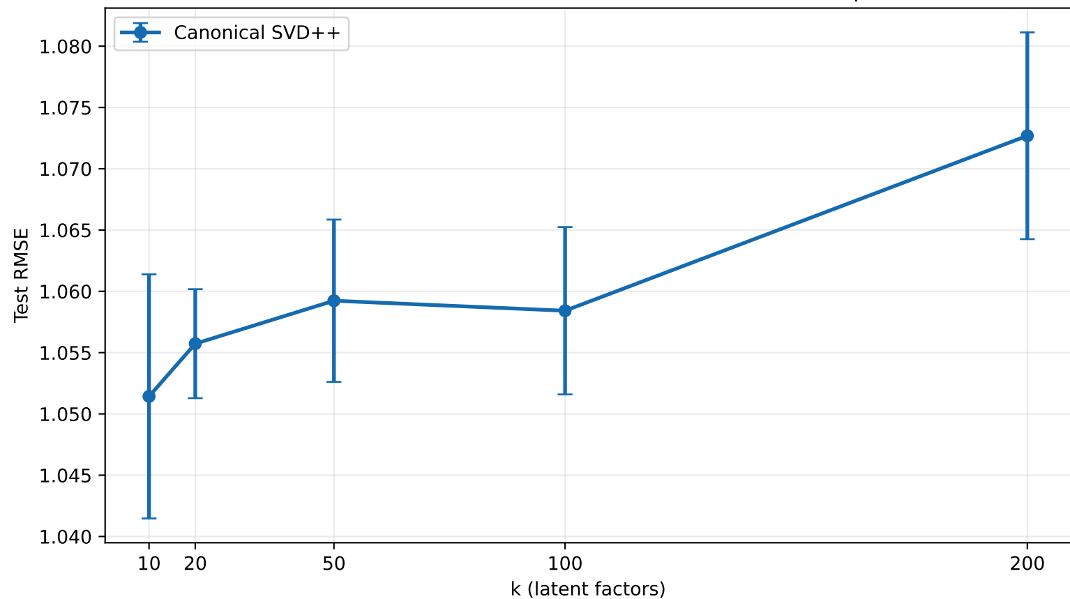
SVD++ — MovieLens 100K subset, fixed random split
