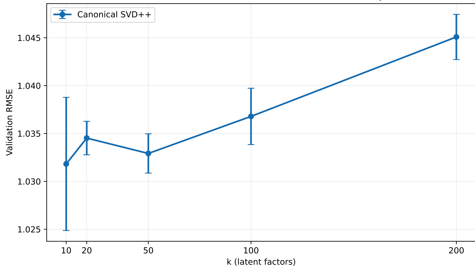
SVD++ — MovieLens 100K subset, fixed random split
