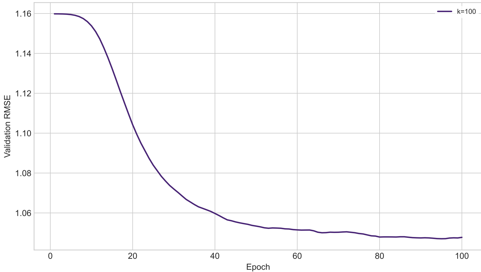
Pure Matrix Factorization: Validation RMSE Training Curves
