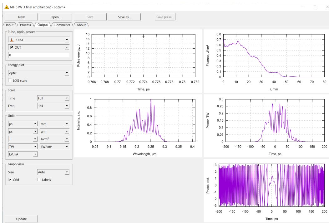
Figure 2.2: "Output" tab of the co2amp+ user interface program. Controls on the left allow selecting the data to display and fine-tuning the look of the plots.
