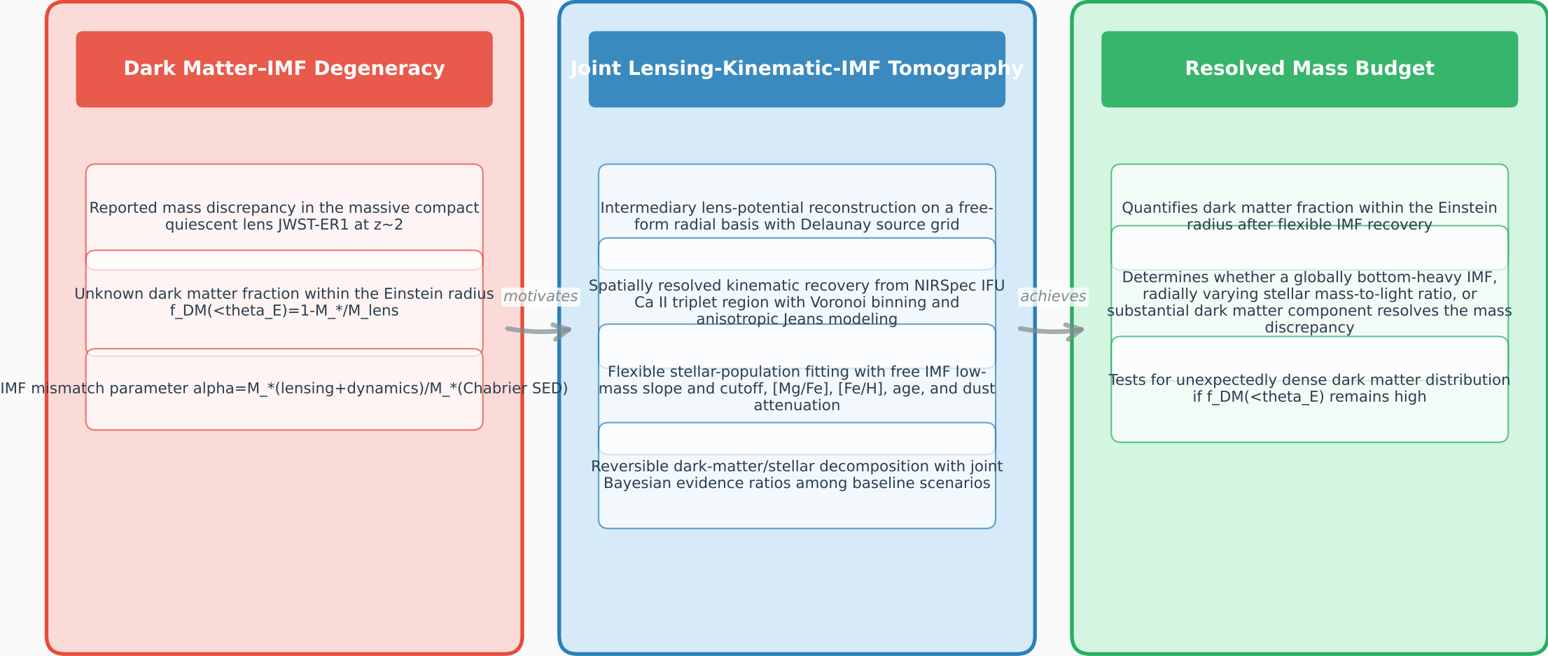
Figure 1: Overview of the JWST-ER1 joint strong-lensing, NIRSpec IFU kinematic, and spectro-photometric IMF tomography framework, in which the dark matter-IMF degeneracy motivates a free-form lens-potential reconstruction and reversible dark-matter/stellar decomposition to quantify the dark matter fraction within the Einstein radius and compare evidence ratios among Chabrier, bottom-heavy, and radially varying IMF scenarios.
