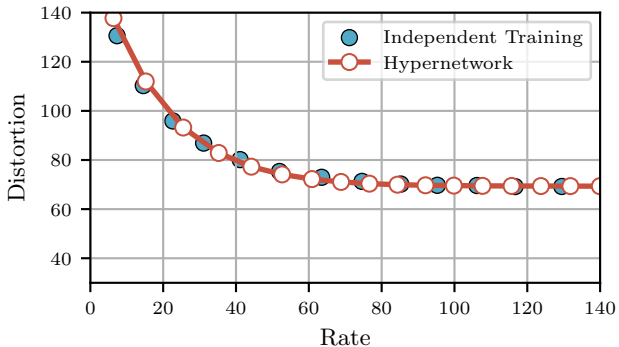
Rate-Distortion Curve for MNIST
