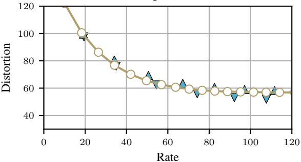
Omniglot Dataset
