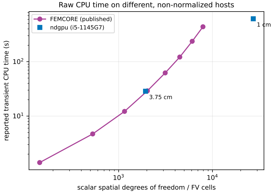
Figure 8: Published FEMCORE and measured ndgpu transient CPU times. The hosts differ and FEMCORE’s hardware is not disclosed; no cross-code speedup is formed.
