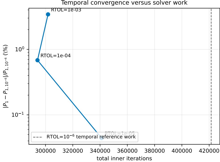
Figure 6: First-peak temporal convergence versus total inner iterations. The dashed line records the cost of the tight temporal reference; it is not plotted as a fictitious nonzero error point.
