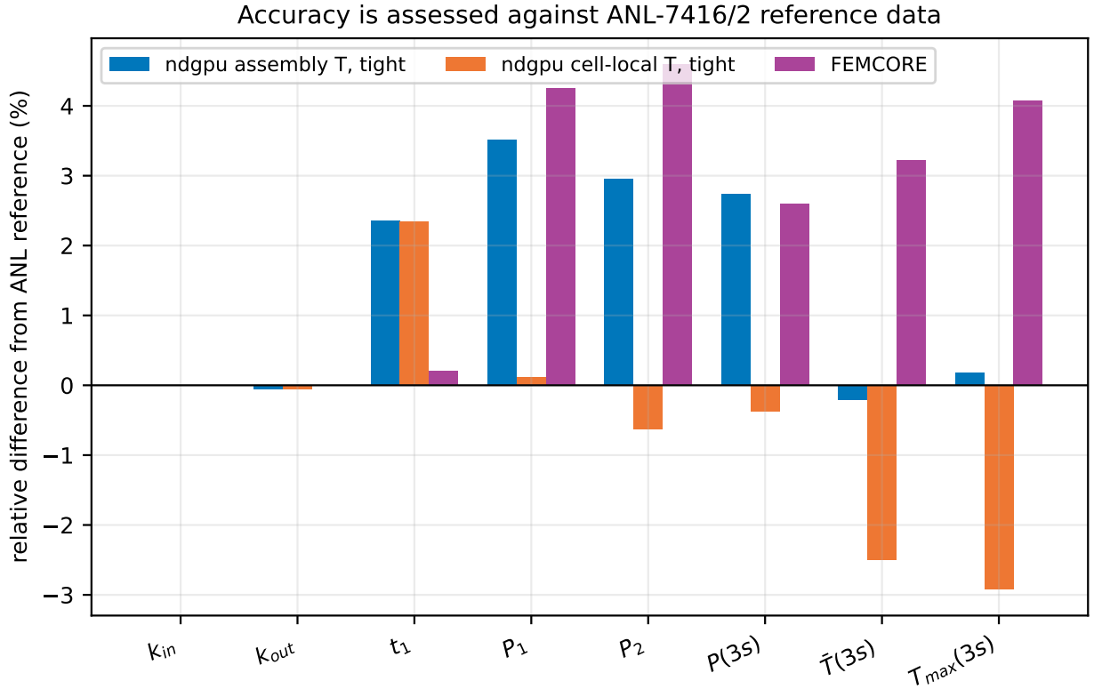
Figure 3: Feedback resolution at fixed 3.75 cm mesh. Cell-local feedback moves all three power values substantially closer to ANL; assembly-averaged feedback remains the appropriate reproduction of Cherezov’s stated approximation. FEMCORE is secondary, not the reference baseline.
