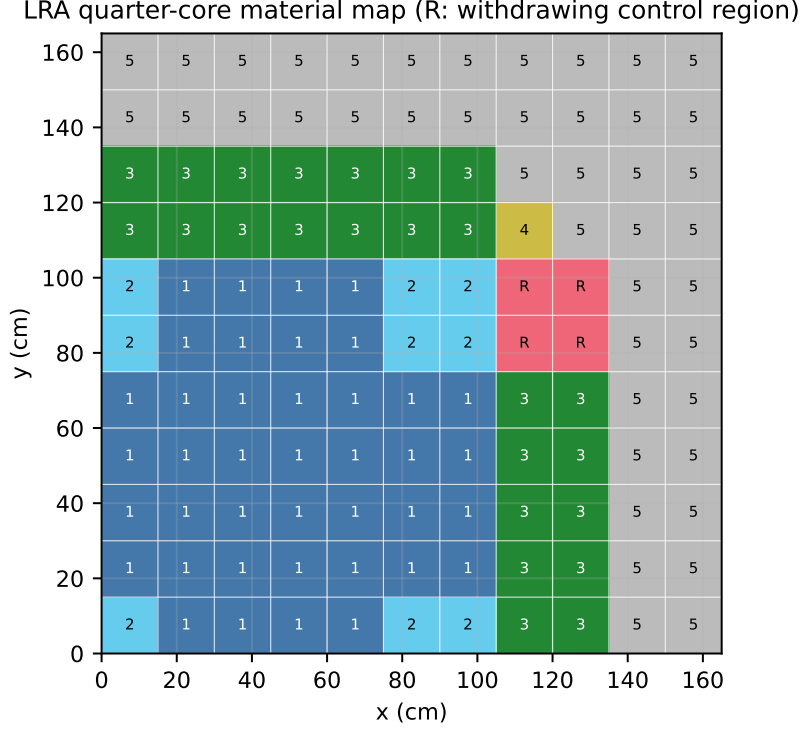
Figure 1: Quarter-core material map used by ndgpu . Region R is the four-cell control region. Performance is measured with four FV cells per assembly edge (3.75 cm); the ANL convergence study extends to fifteen (1 cm).
