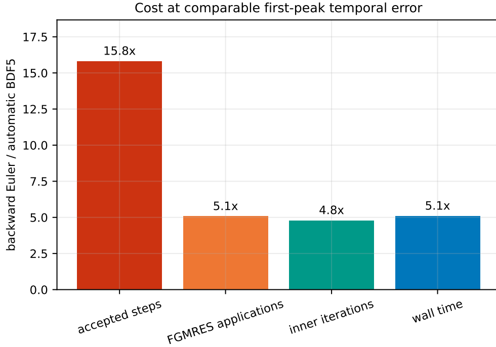
Figure 7: Backward-Euler cost divided by automatic-BDF5 cost at comparable first-peak temporal error. Work-counter ratios are more portable than the single-host wall-time ratio.
