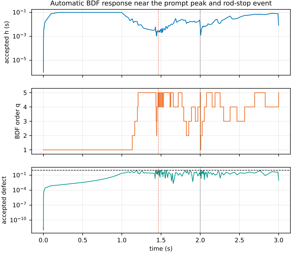
Figure 2: Accepted step width, selected order, and normalized accepted defect for the practical automatic-BDF run ( \text{RTOL} = 10^{-3} ). The red dotted line is the first power peak; the black dotted line is the 2 s rod-stop event. The controller contracts to millisecond steps near both rapid changes and recovers large steps in smooth intervals.
