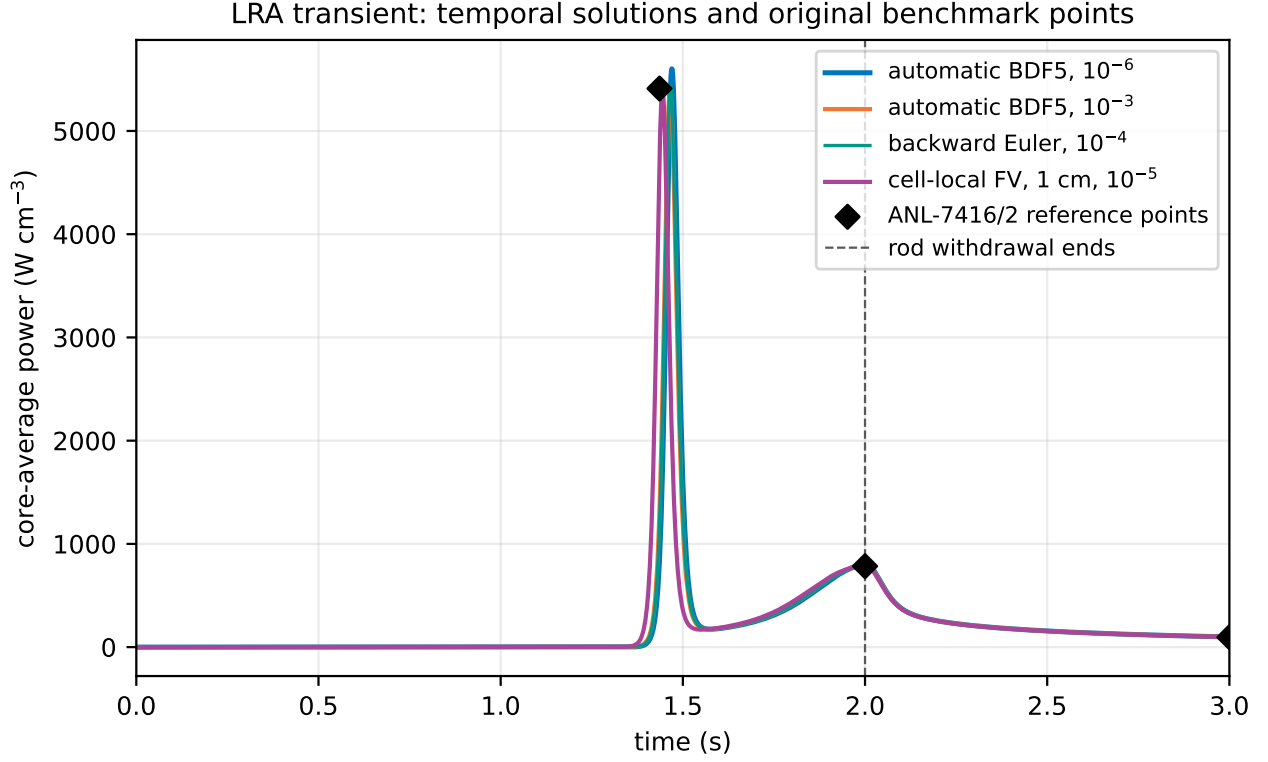
Figure 4: Complete accepted power histories with the three original ANL point references. The black line marks the end of linear control withdrawal. The 1 cm cell-local curve is the spatially refined validation result; the other curves support the fixed-mesh performance comparison.
