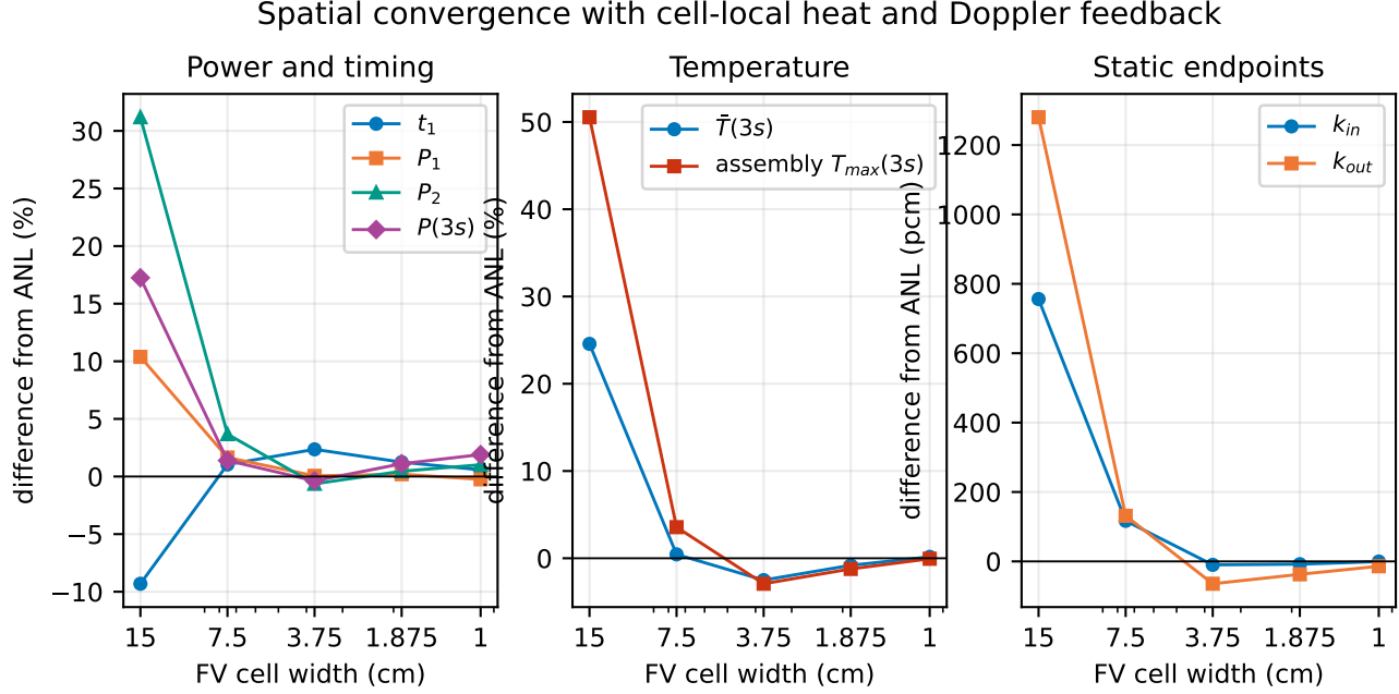
Figure 5: Signed spatial convergence against ANL using cell-local heat and Doppler feedback. Peak temperature denotes the maximum assembly average.
