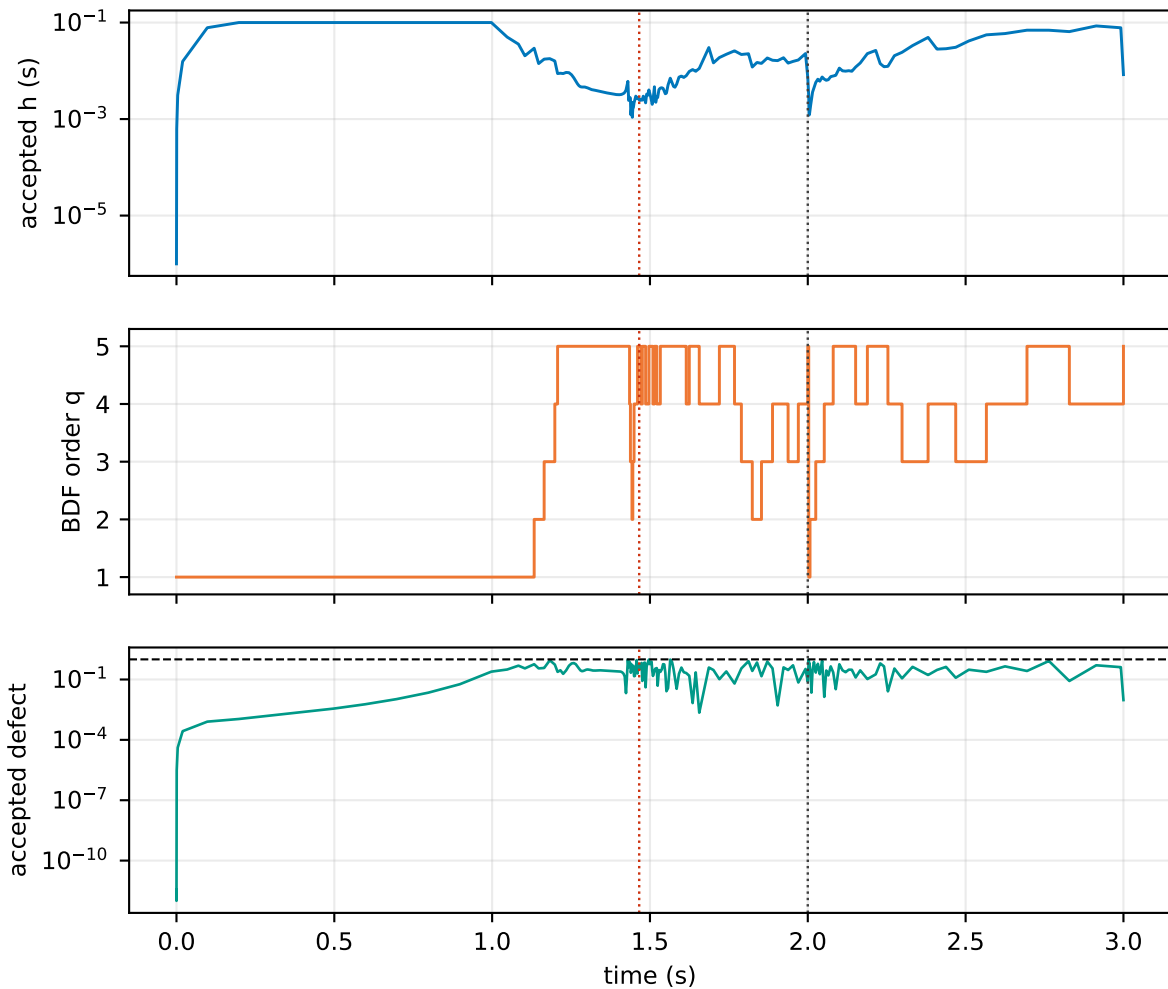
Automatic BDF response near the prompt peak and rod-stop event
