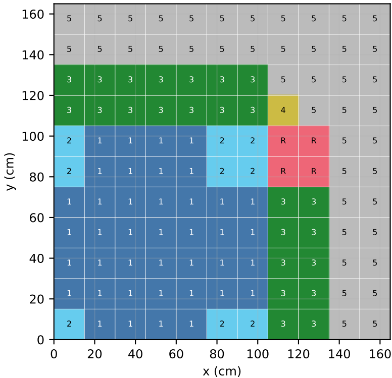
LRA quarter-core material map (R: withdrawing control region)
