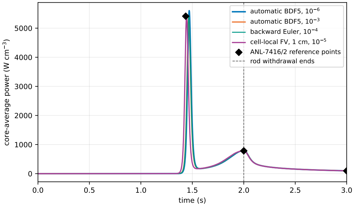
LRA transient: temporal solutions and original benchmark points
