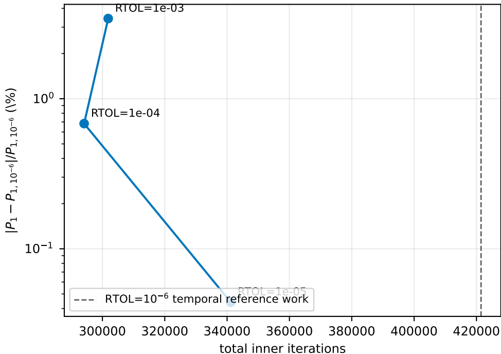
Temporal convergence versus solver work
