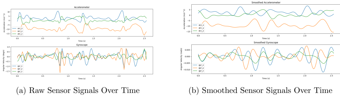
Figure 2: Time-series sensor signal examples
