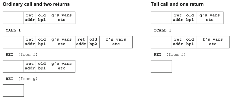
Fig. 12.1 Example replacement of a call and a return by a tail call. On the left , g calls f by the CALL instruction, f returns to g , and g returns to its caller. On the right , g calls f by the TCALL instruction, discarding g 's stack frame but keeping its return address and old base pointer, so that f returns straight to g 's caller
