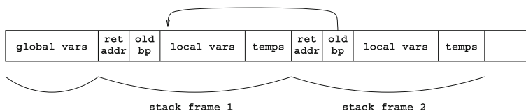
Fig. 8.2 Stack layout at run-time
