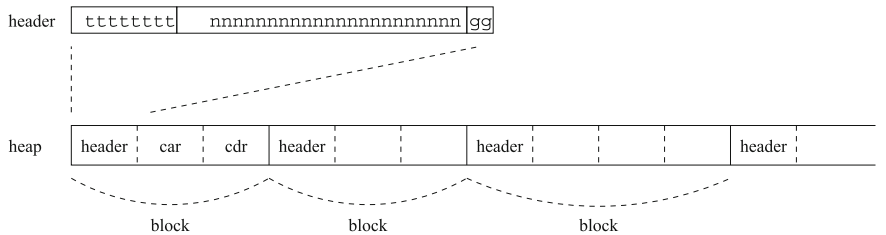
Fig. 10.5 The list-C run-time heap is covered by blocks. Each block consists of a header word and n \geq 0 other words, each being 32 bits. A header is divided into 8 tag bits, 22 size bits (representing n ), and 2 garbage collection bits
