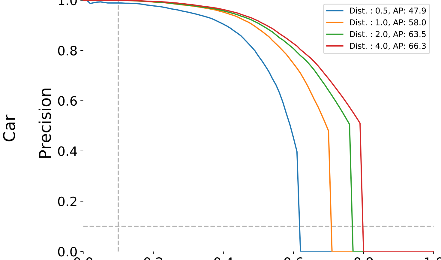
Recall vs Precision
