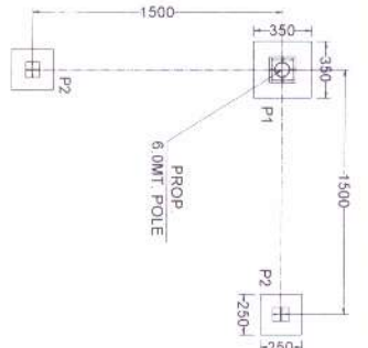
PROP R.T.P. 6.0M. POLE (AS PER RIL DRG. NO. :- 10070-118-635/10659-B02-075)
