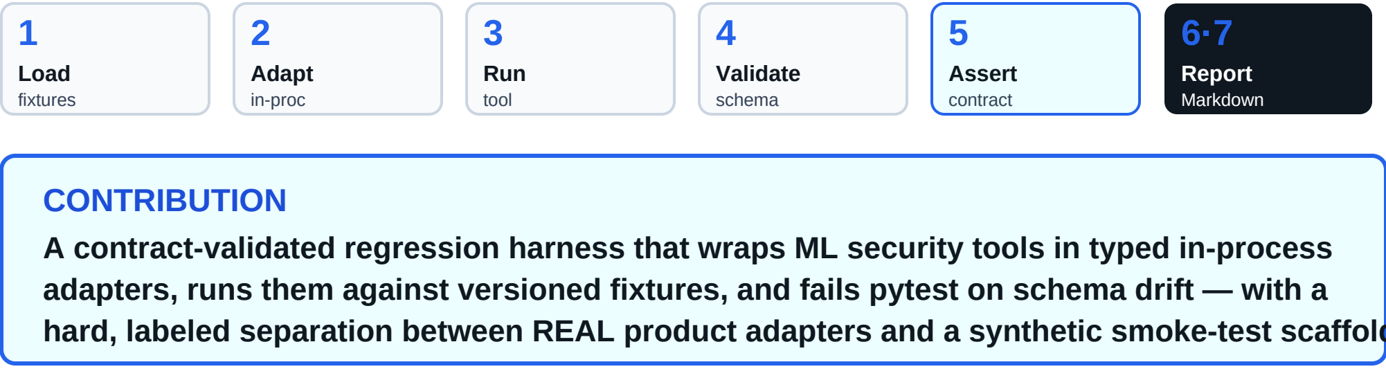
Figure 1. Typed adapters run tools in-process against frozen fixtures and validate outputs against a shared schema; drift fails pytest.
