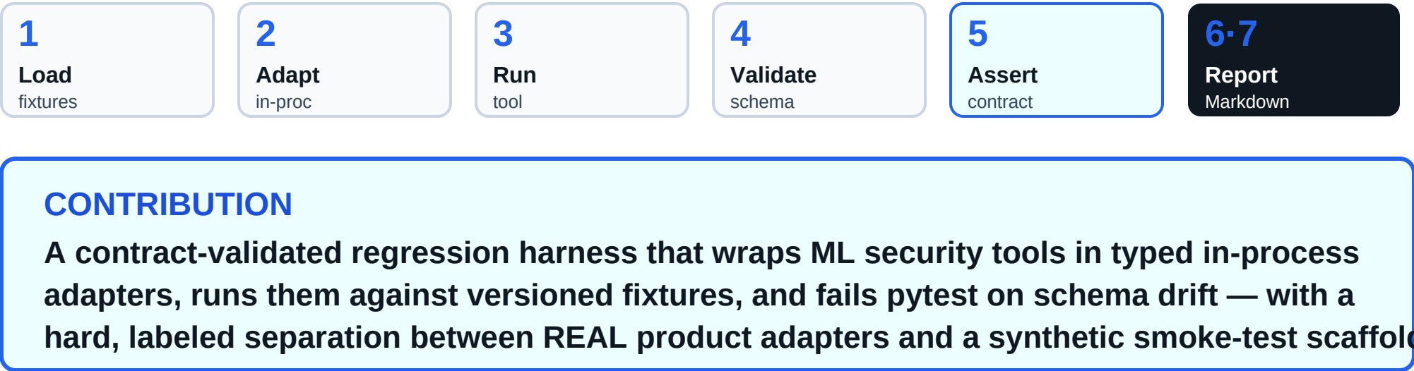
Figure 1. Typed adapters run tools in-process against frozen fixtures and validate outputs against a shared schema; drift fails pytest.
