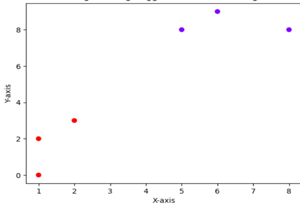
Single Linkage Agglomerative Clustering
