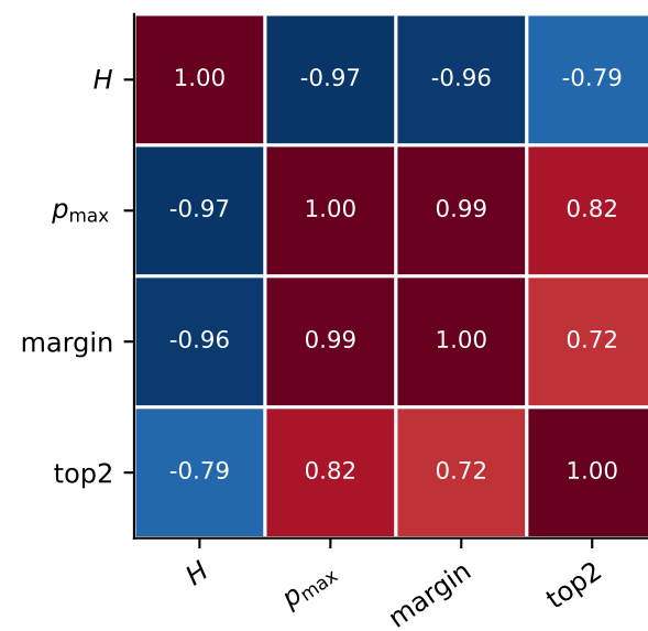
Within weak H / p_{\max} family
