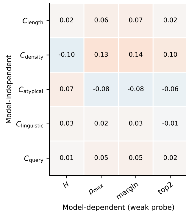
Cross: C_* \times weak model-dependent (pooled)
