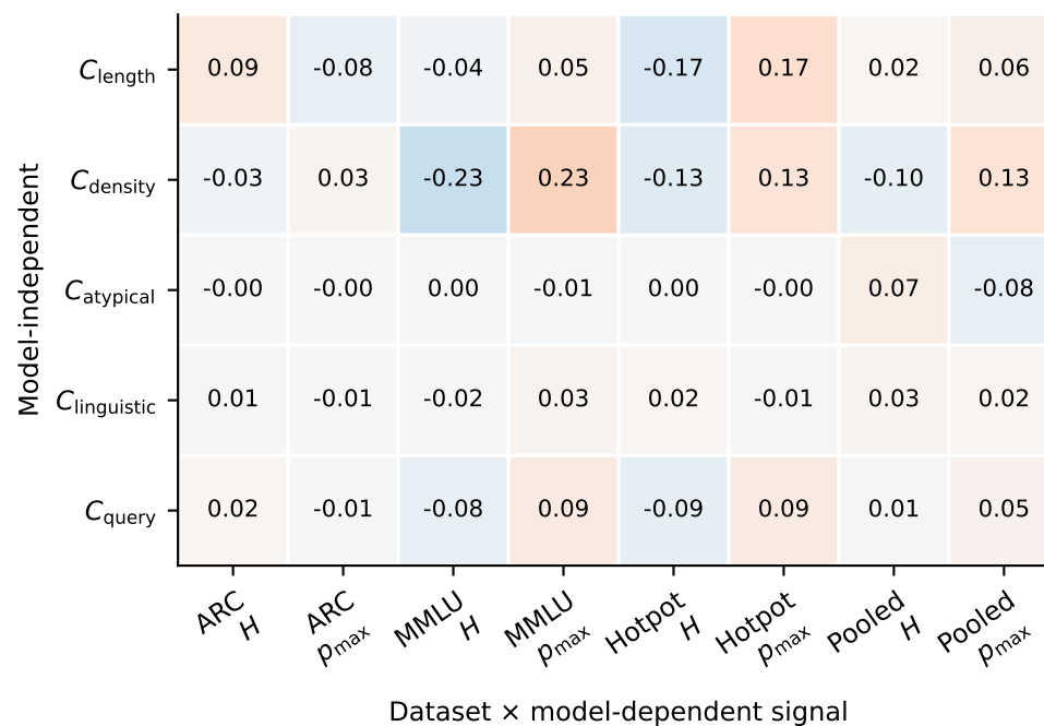
C_* \times weak H / p_{\max} by dataset
