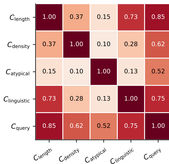
Within C_* (pooled)
