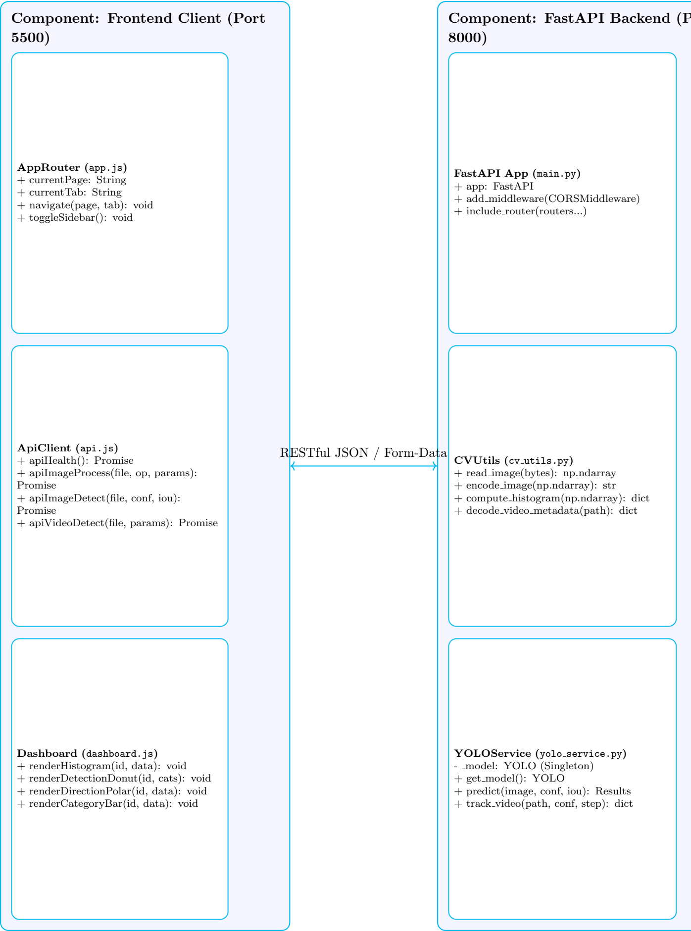
Figure 5: Component and Class Dependency Architecture of VisionLab. 16
