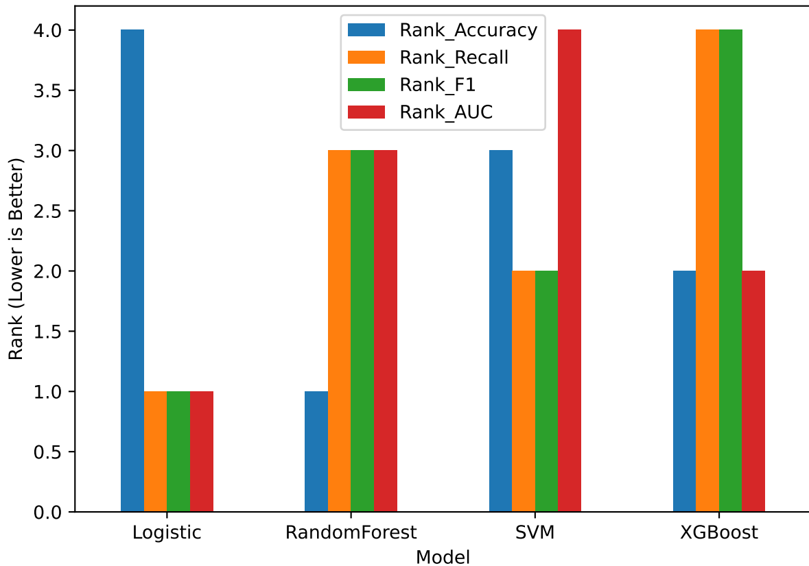
Model Ranking Across Metrics
