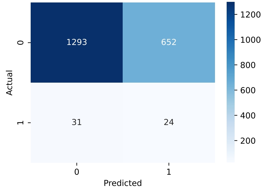
Logistic Regression
