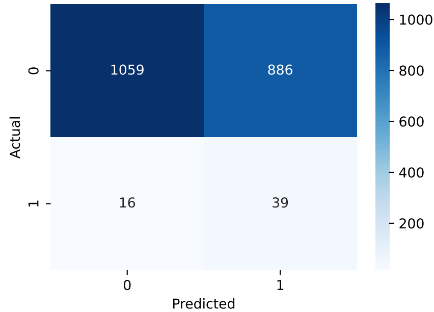
Decision Tree
