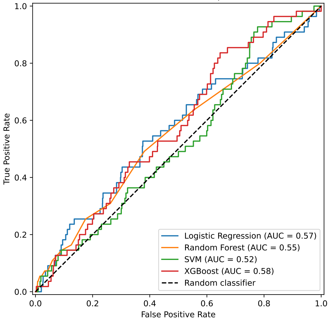
RQ2 — ROC Curve Comparison
