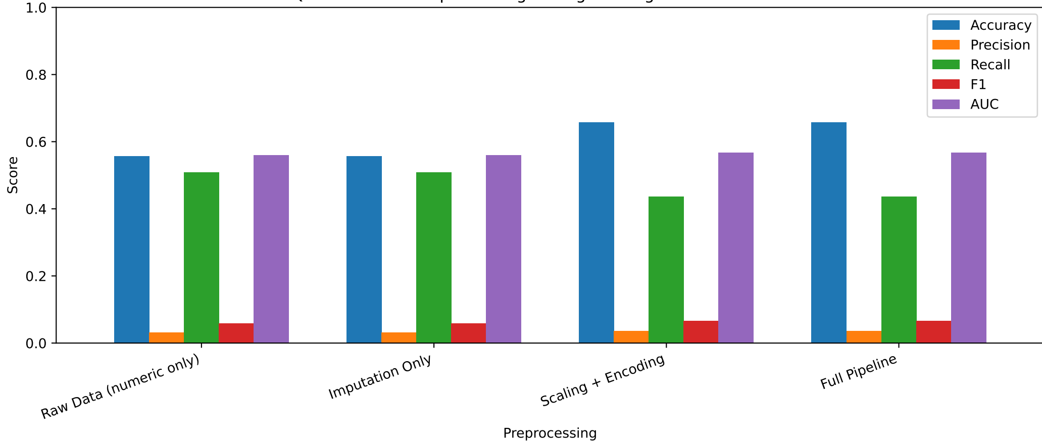
RQ3 — Effect of Preprocessing on Logistic Regression Performance
