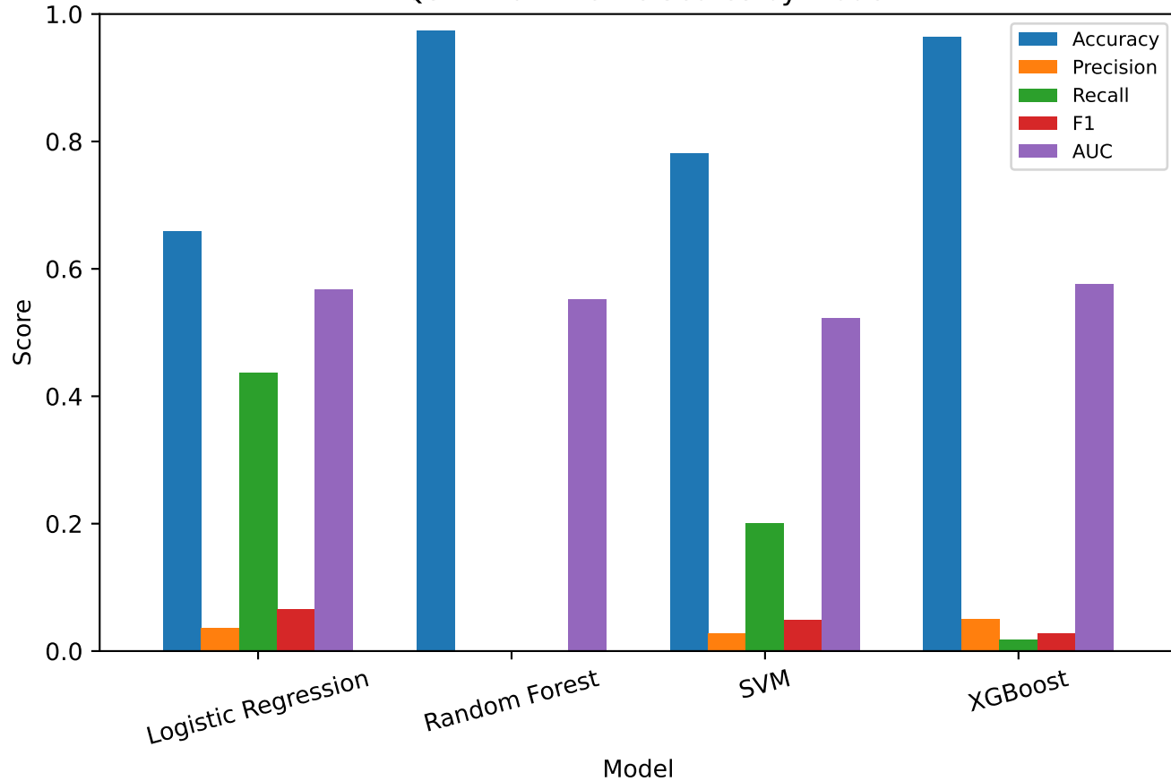
RQ5 — Raw Metric Scores by Model
