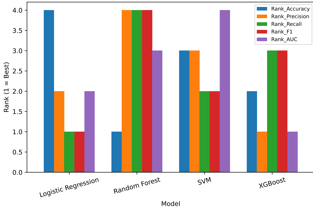
RQ5 — Per-Metric Ranks (Lower = Better)
