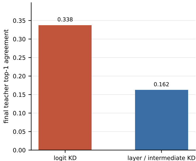
b Teacher imitation — higher is better
