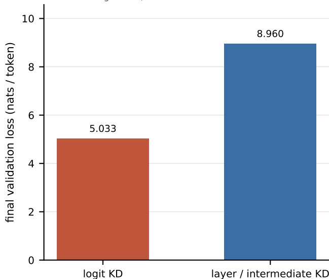
a Held-out loss — lower is better
