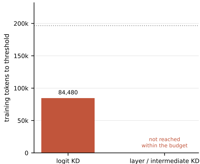
b Tokens to top-1 agreement \geq 0.3
