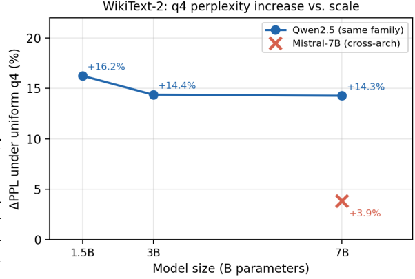
Figure 4: Perplexity increase (%) under uniform q4 quantization versus model parameter count (WikiText-2). Within the Qwen family (filled circles), \Delta PPL is nearly flat: +16.2% (1.5B), +14.4% (3B), +14.3% (7B). Mistral-7B (cross marker) degrades only +3.9% at the same 7B scale, a 3.7 \times cross-architecture gap. All models share \approx 3.5\times compression.
