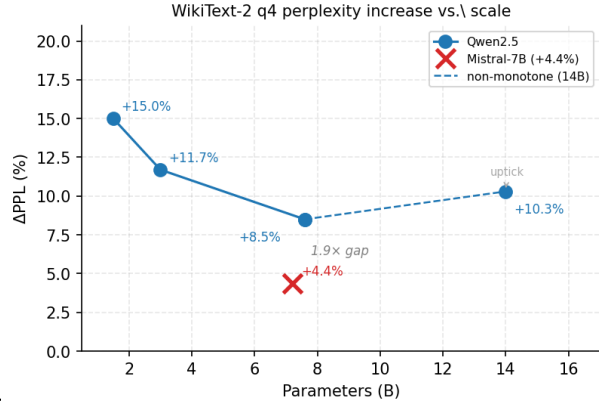
Figure 4: (q4) Perplexity increase (%) under uniform q4 quantization versus model parameter count (WikiText-2). Within the Qwen family (filled circles), \Delta\text{PPL} under uniform local-pipeline q4: +15.0% (1.5B), +11.7% (3B), +8.5% (7B), +10.3% (14B). The 14B result is slightly above 7B. Mistral-7B (cross marker) degrades only +4.4% at the same scale, a 1.9\times cross-architecture gap. All models share \approx 3.5\times compression.
