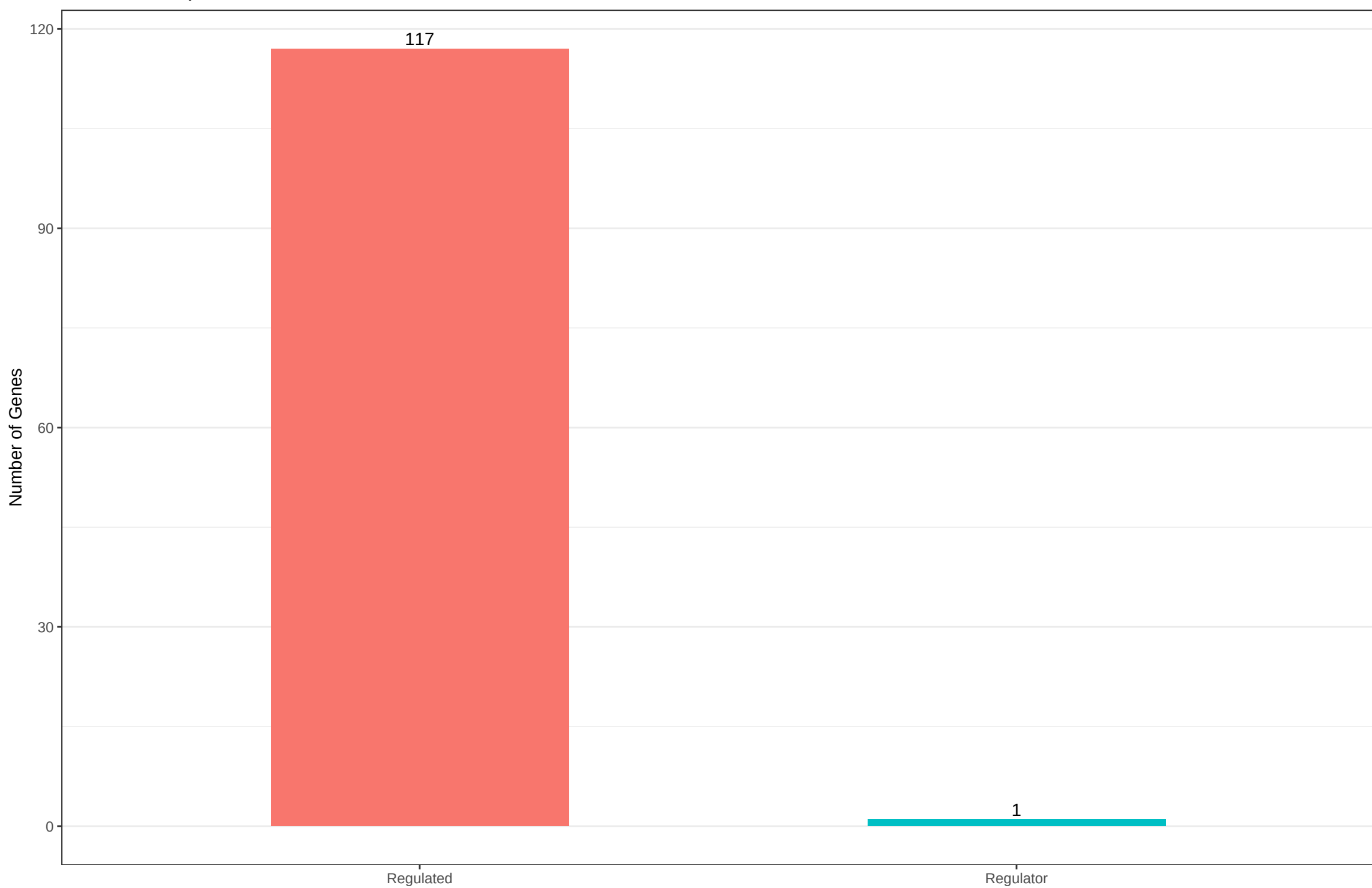
Network Composition – C4–GATA–related
