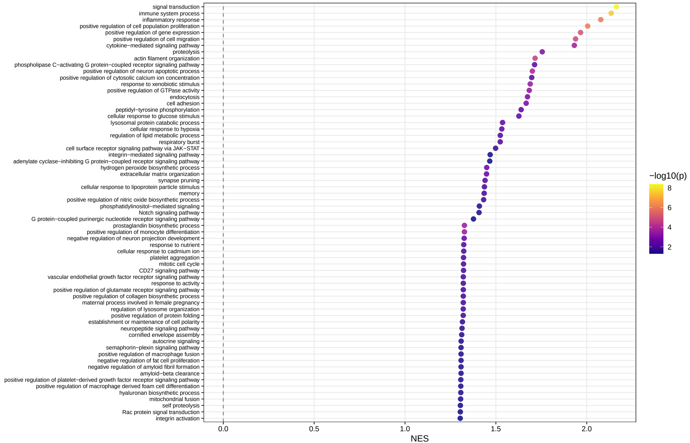
GO:BP fgsea – C4–GATA-related (65 terms)
