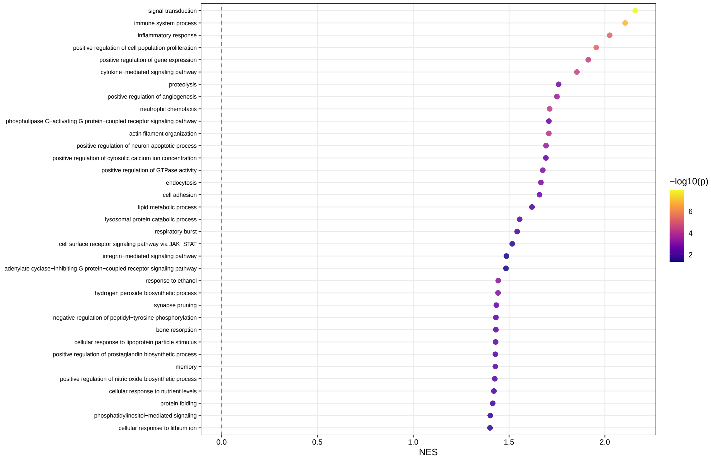
GO:BP GSEA – C4–GATA–related (35 terms)
