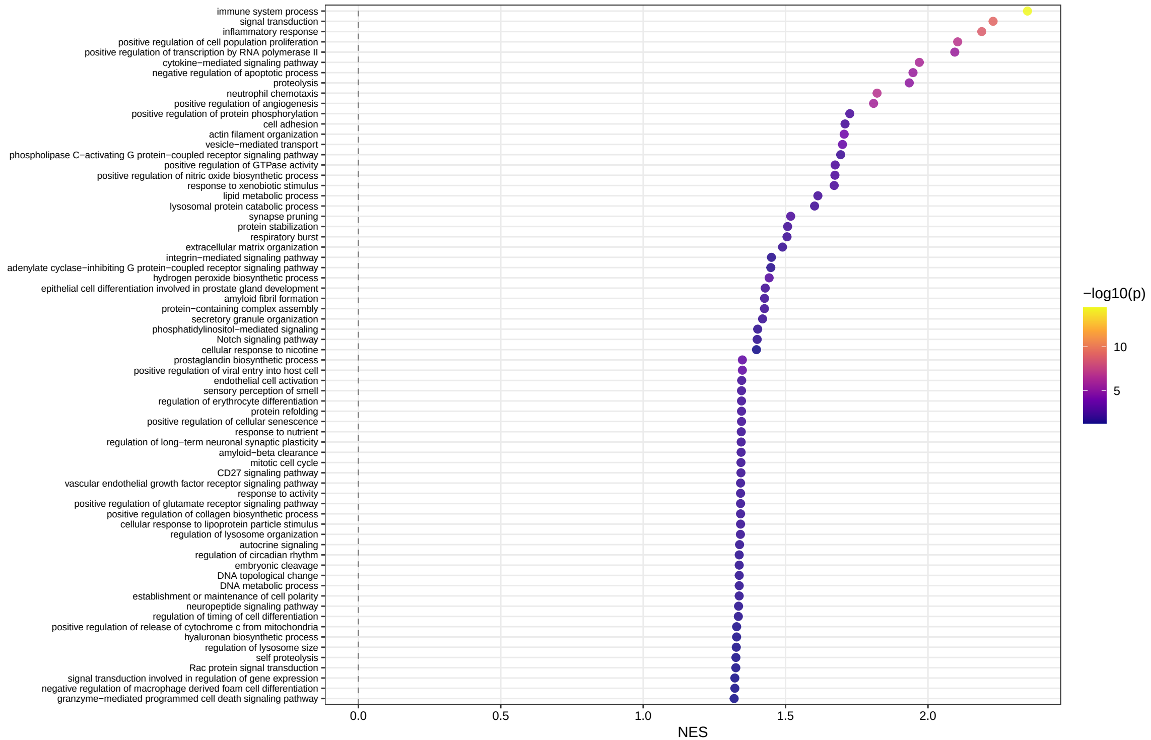
GO:BP fgsea – STAT factors (68 terms)
