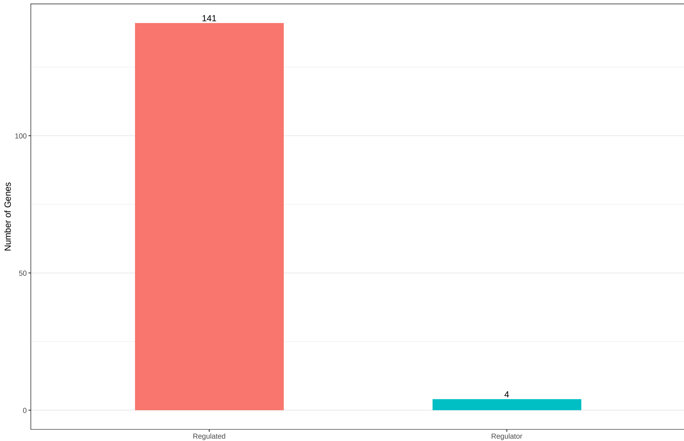
Network Composition – STAT factors
