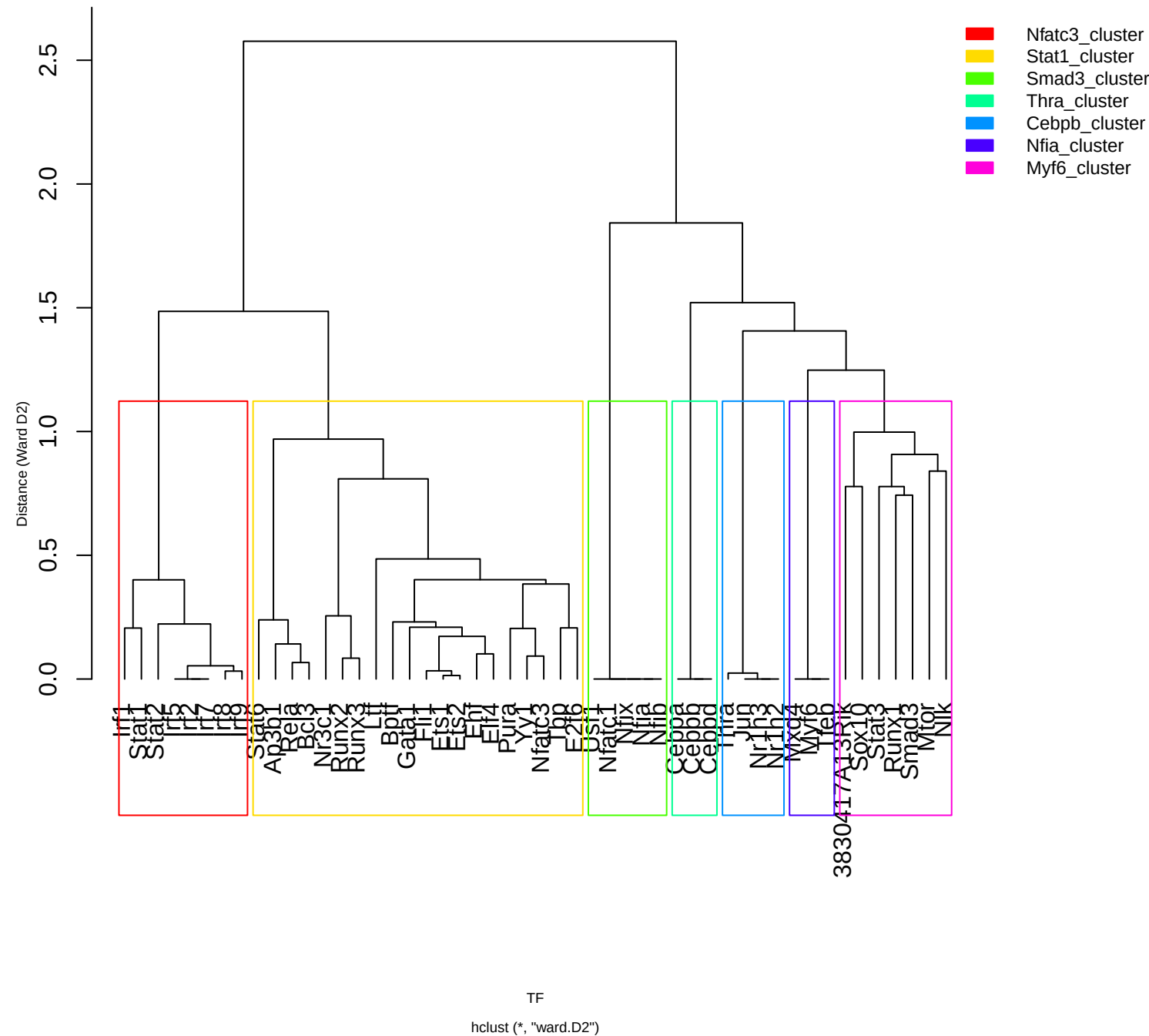
Dendrogram – Jaccard (h = 1.00, 7 clusters)
